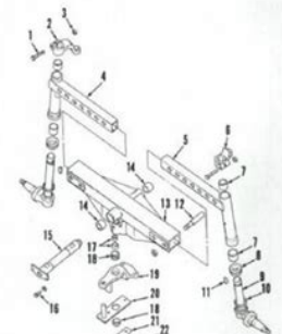
Fig. 3—Exploded view of straight adjustable front axle used on some tractors.
