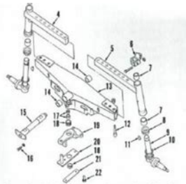
Fig. 4—Exploded view of heavy duty straight adjustable front axle used on some tractors. Refer to Fig. 3 for legend.
